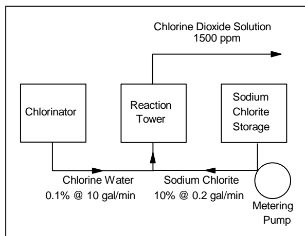
Figure 1 Chlorine Dioxide Generator
