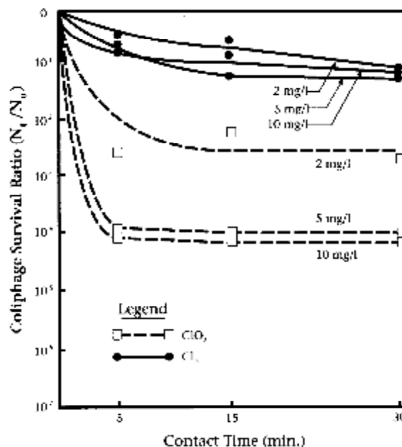
In situ coliphage survival in secondary effluent at three doses and three contact times
