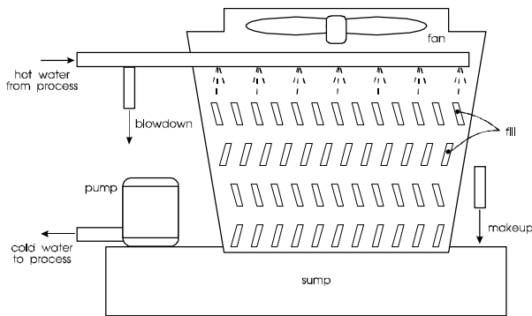
Figure 1 - Cooling Tower
